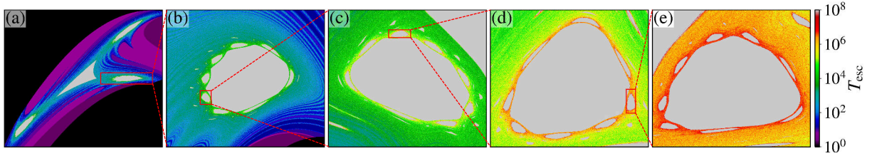
Figure 4.7: The escape time for a grid of 1000 \times 1000 uniformly distributed initial conditions in the regions given in Table 4.1 for the standard map with k = 6.908745 . Figures (b)-(e) are magnifications around the indicated islands and the color bar is in logarithmic scale.
