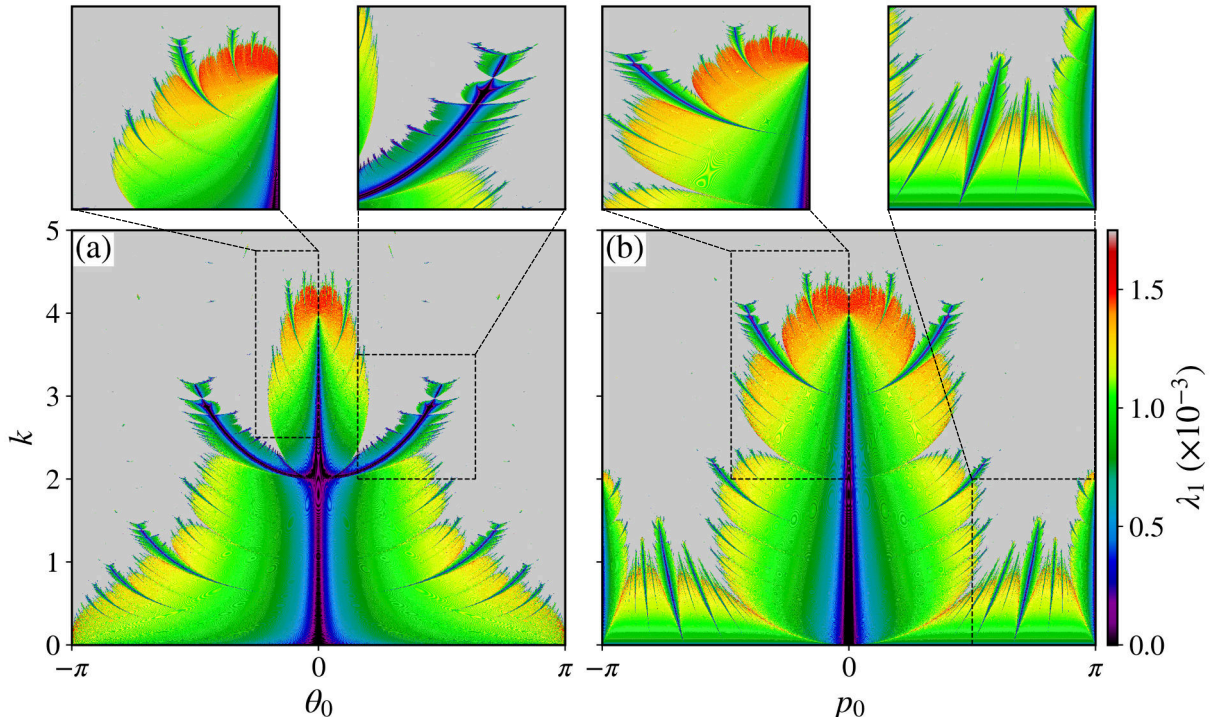
Figure 3.7: The largest Lyapunov exponent for a 1000 \times 1000 grid of uniformly chosen values of (a) (k, \theta_0) with p_0 = 0 , and (b) (k, p_0) with \theta_0 = 0 and T = 1.0 \times 10^4 .
