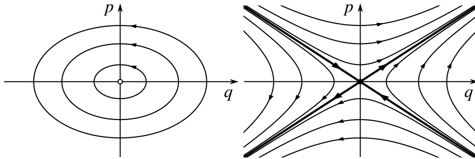
Figure 2.5: Neighborhood of an elliptic point (on the left) and a hyperbolic point (on the right). The orbits that circle about the elliptic point in elliptical trajectories are called elliptical orbits. The thinner lines in the figure on the right represent hyperbolic orbits that move away from the hyperbolic point in all directions. The thicker lines are the asymptotes (stable and unstable directions) of the hyperbolic point.
