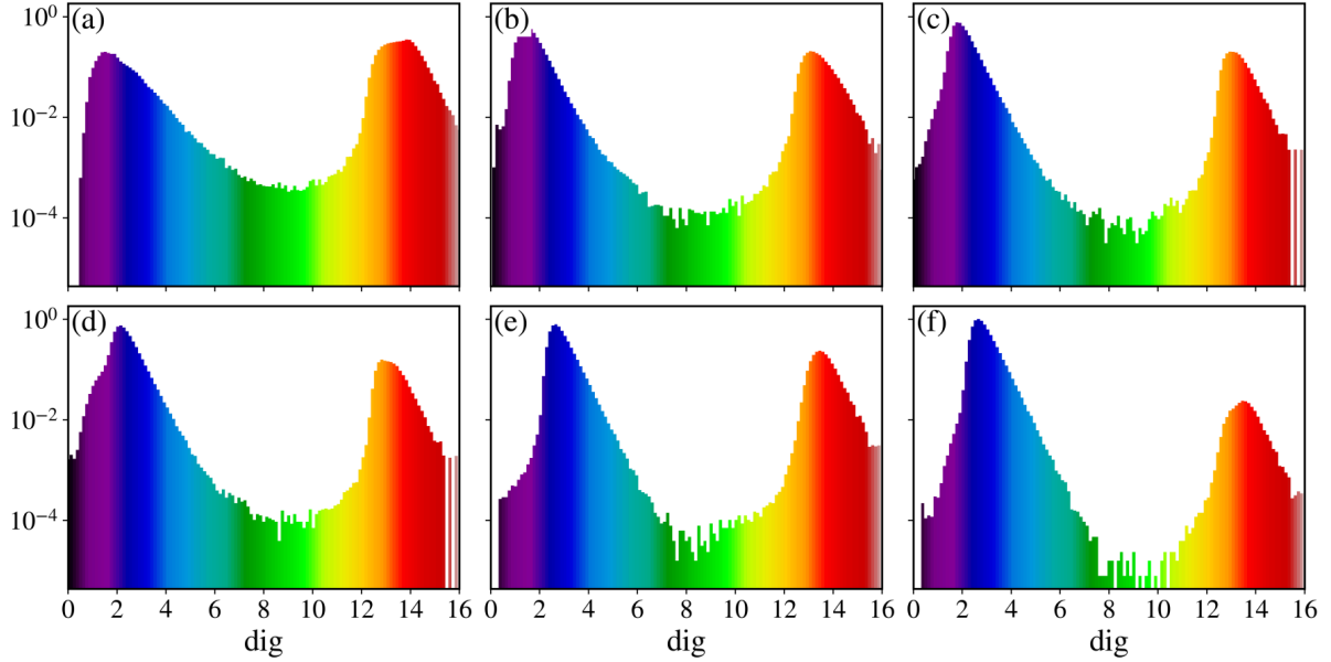
Figure 4.2: Histograms of the values of \text{dig} shown in Figure 4.1. There are mainly two peaks, each one characterizing one dynamical regime. The peak for small values of \text{dig} corresponds to chaotic orbits, while the peak for larger values of \text{dig} to regular orbits. There are orbits with an intermediate value of \text{dig} , and they are trapped orbits whose value of \text{dig} has yet not converged its asymptotic value. We note that as k increases, the proportion of regular orbits diminishes, as expected.
