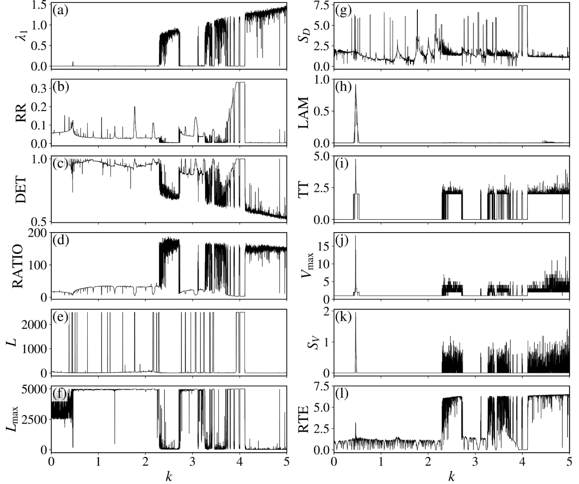
Figure 5.3: (a) The largest Lyapunov exponent, (b) the recurrence rate, the RQA measures (c)-(g) based on diagonal lines, given by Eqs. (5.12)-(5.16), respectively, and (h)-(k) based on vertical lines, given by Eqs. (5.18)-(5.21), respectively, and (l) the recurrence time entropy [Eq. (5.23)] as a function of the nonlinearity parameter k , with a step of \Delta k = 0.001 . The length of the time series is N = 5000 , and for each parameter value, we choose a fixed initial condition of (\theta_0, p_0) = (0.0, 1.3) .
