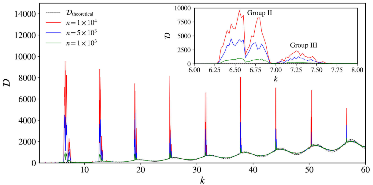
Figure 3.8: The diffusion coefficient, Eq. (3.45), for the standard map as a function of the nonlinearity parameter, with \Delta k = 0.025 for (green) n = 1.0 \times 10^3 , (blue) n = 5.0 \times 10^3 , and (red) n = 1.0 \times 10^4 . In black dashed line is the theoretical value for the standard map as predicted in (3.44). We considered 100 \times 100 initial conditions uniformly distributed in a grid on the entire phase space [0, 2\pi] \times [0, 2\pi] . Inset: magnification on the interval k \in [6, 8] that shows the groups II and III of accelerator mode islands. We observe a deviation of the numerically calculated diffusion coefficient from its theoretical value.
