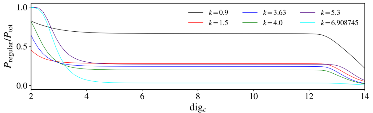
Figure 4.3: The normalized proportion of regular orbits as a function of the cutoff value \text{dig}_c for the data in Figures 4.1 and 4.2. For small and large values of \text{dig} , the proportion changes significantly, however, there is an interval around \text{dig}_c \in [5, 12] in which the proportion is almost constant.
